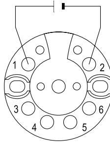
POWER SUPPLY
